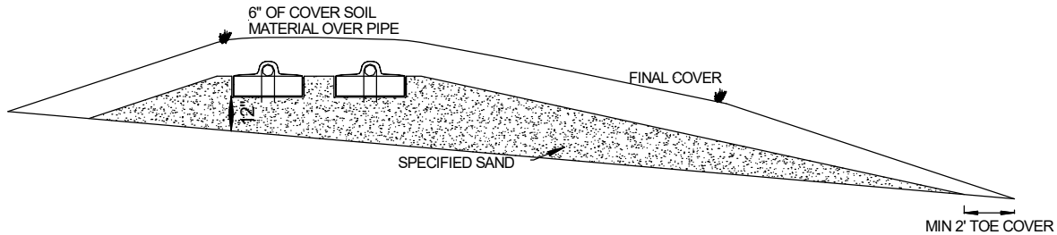
FIGURE 13: SLOPED ABOVE GRADE BED CROSS SECTION
