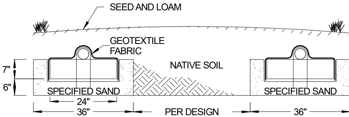
FIGURE 5: SECTION VIEW – TRENCH SYSTEM – SLOPING SITE
