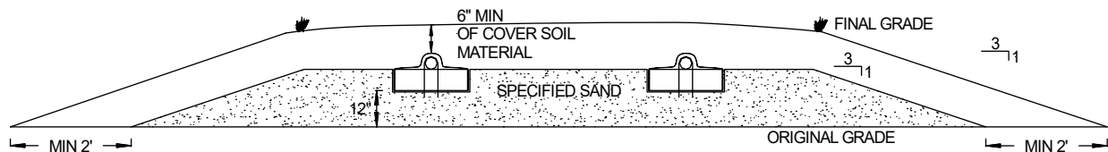
FIGURE 10: LEVEL ABOVE GRADE CROSS SECTION
