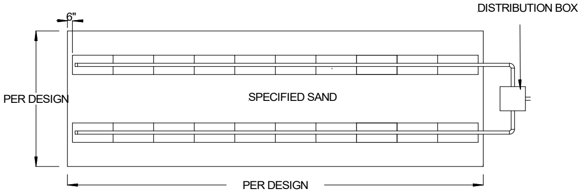
FIGURE 7: PLAN VIEW – BED SYSTEM
