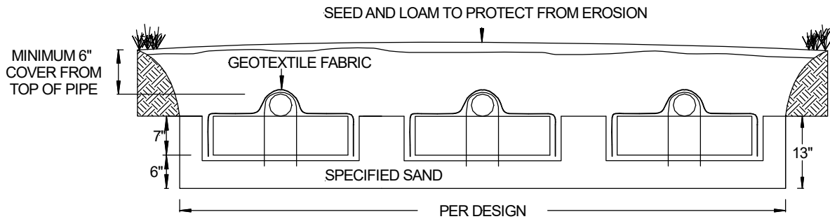
FIGURE 9: SECTION VIEW – 3 LATERAL BED SYSTEM
