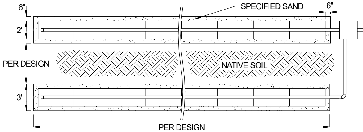
FIGURE 3: PLAN VIEW – TRENCH SYSTEM
