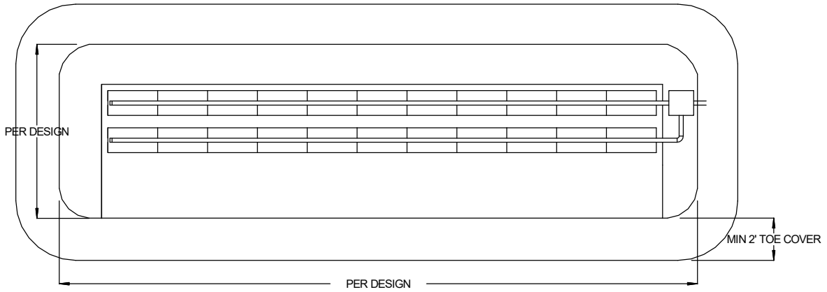
FIGURE 14: PLAN VIEW – BED SYSTEM –SLOPING SITE
