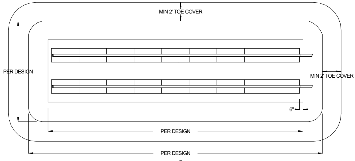
FIGURE 11: PLAN VIEW – BED SYSTEM – LEVEL SITE
