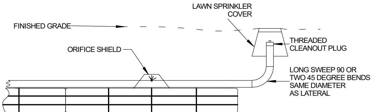
FIGURE 16: PRESSURE CLEAN OUT
