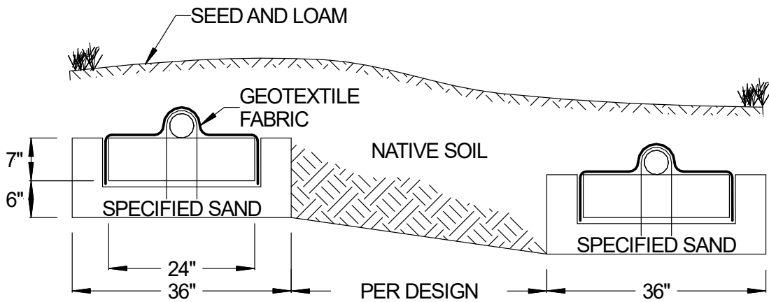
FIGURE 5: SECTION VIEW – TRENCH SYSTEM – SLOPING SITE
