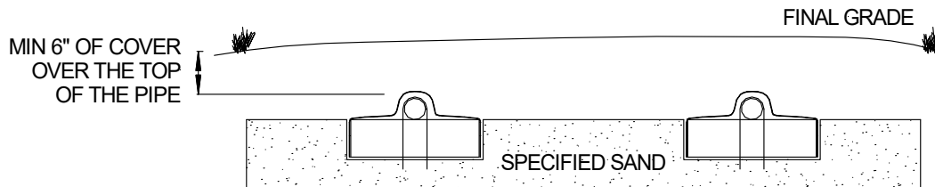
FIGURE 6: BED CROSS SECTION
