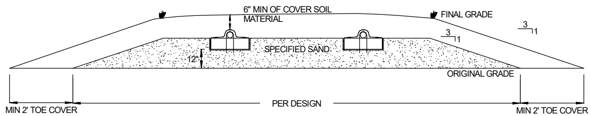
FIGURE 12: CROSS SECTION VIEW – BED SYSTEM – LEVEL SITE
