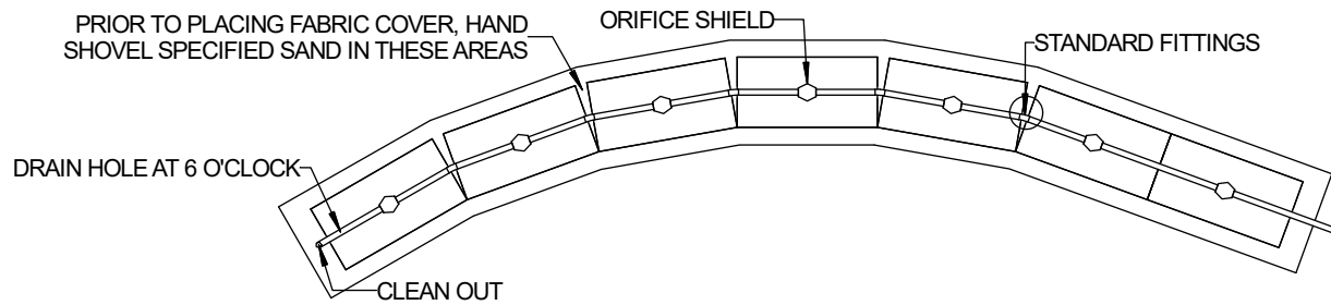
FIGURE 17: CONTOURED TRENCH PRESSURE DISTRIBUTION
