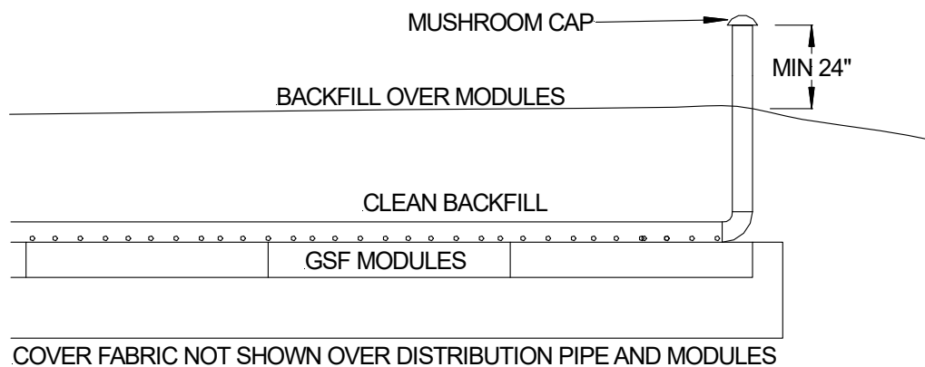
FIGURE 18: GSF WITH 4" VENT EXTENDED TO CONVENIENT LOCATION
