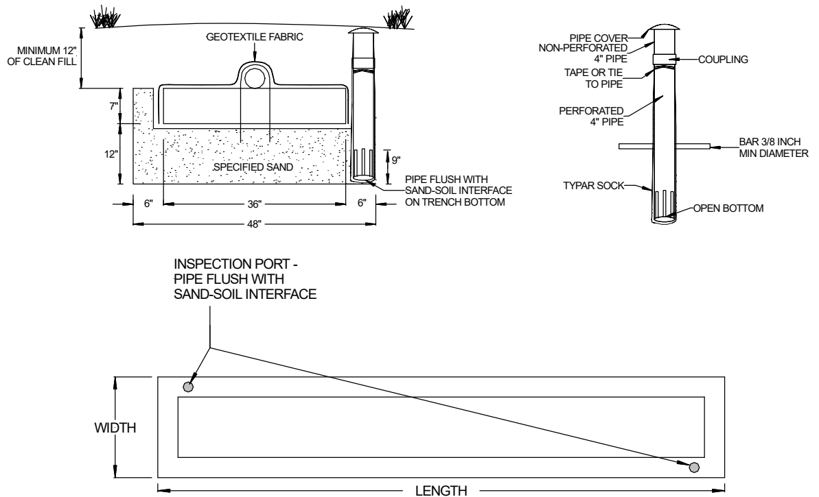
Figure 8. Observation pipes
